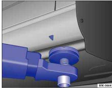
Fig. 146 Front lift point for workshop hoist or floor jack.
