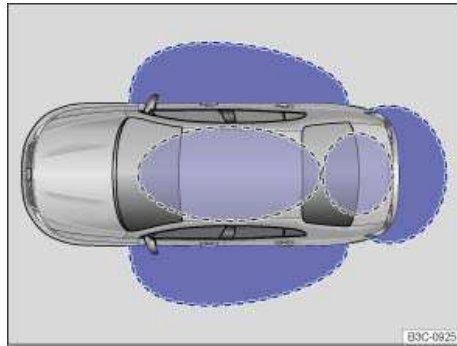
Fig. 22 Ranges of the Keyless Access locking and starting system. Outside the vehicle: Unlocking range. Inside the vehicle: Starting range.
