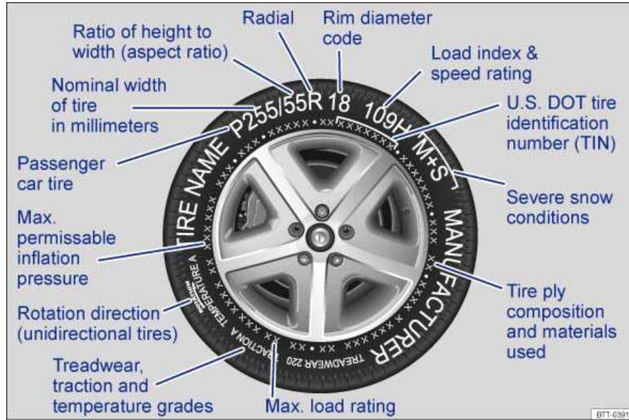
Fig. 93 International tire labeling.
