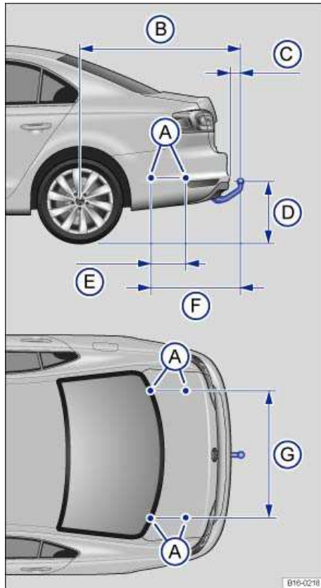
Fig. 87 Dimensions and attachment points for retrofitting a trailer hitch.
