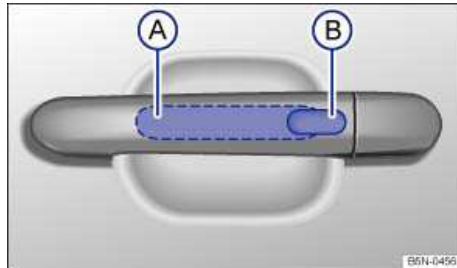
Fig. 23 Keyless Access locking and starting system: Sensor for unlocking A on the inside of the front door handles. Sensor for locking B on the outside of the front door handles.
