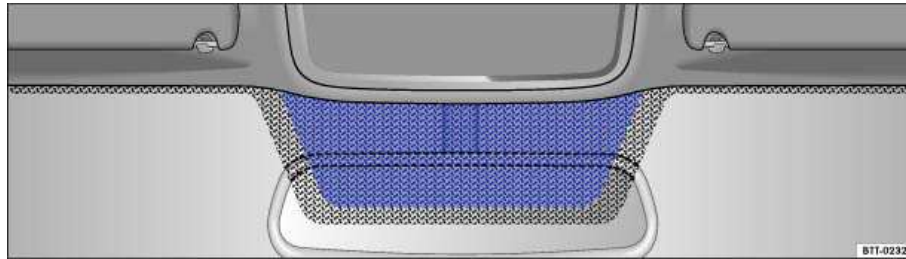
Fig. 74 Heat-reflective windshield with communications window (blue shaded area).
