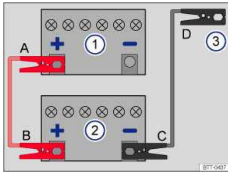
Fig. 180 Diagram for attaching the jumper cables: Dead battery 1 and booster battery 2.
