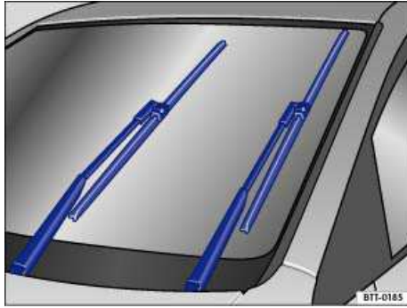
Fig. 76 Windshield wiper in service position.
