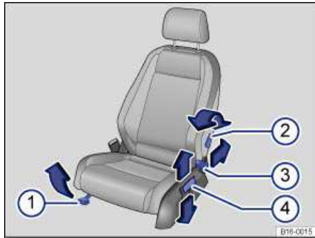
Fig. 34 Driver seat: Manual controls to move the seat forward or back and adjust the backrest angle, seat height, and lumbar support (if applicable).
