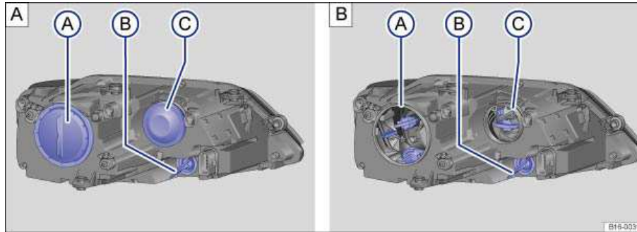
Fig. 172 In the engine compartment: Covers in the left headlight assembly. A Low beam headlight, daytime low beam headlight or daytime running light, side marker light; B Turn signal indicator; C High beam, parking light, daytime running light.
