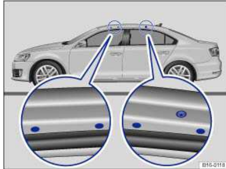
Fig. 85 Attachment points for the base carrier and roof rack.
